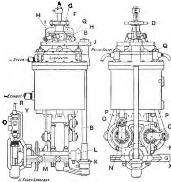
FIG. 266.—Diagram of the "Reading" Steam Carriage Engine. A, rotary valve spindle; B, vertical shaft driving rotary valve; C, suction box of pump; D, split collar of reversing gear; E, stop collar; F, yoke operating bell crank levers for rotating valves and reversing; G, bossed collar carrying bell cranks, H, H, which drive valve, also rotate it to reverse engine; I, spur wheel operating main valve; J, valve pinion; K and L, bevel gears for driving main valve; M, main shaft; N, N, crank shafts; O, O, roller bearings; P, P, P, P, connecting rods of the four cylinders; Q, valve casing; R, feed pump control rod; Y, yoke holding pump; X, stay pivot for chain tightening rod.
